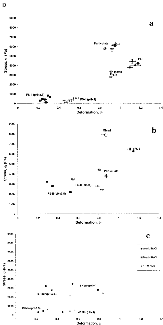
Figure 1. (a) Gel-type determination for 45 min gels using vane fracture. (b) Gel-type determination for 3 h gels using vane fracture. (c) Vane of 45 min and 3 h FS–II gels.
